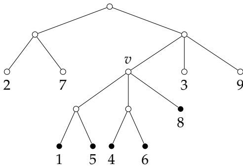
(a) Leaves in \sigma -order, labeled with \rho -ranks
